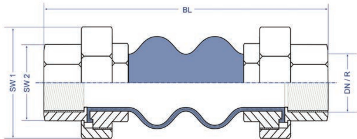
Rubber-Expansion-Joint Type 200 /Y /O
