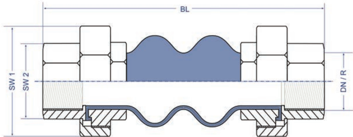
Rubber-Expansion-Joint Type 200 /Y /O
